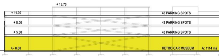
SECTION A-A 129 PARKING SPOTS
