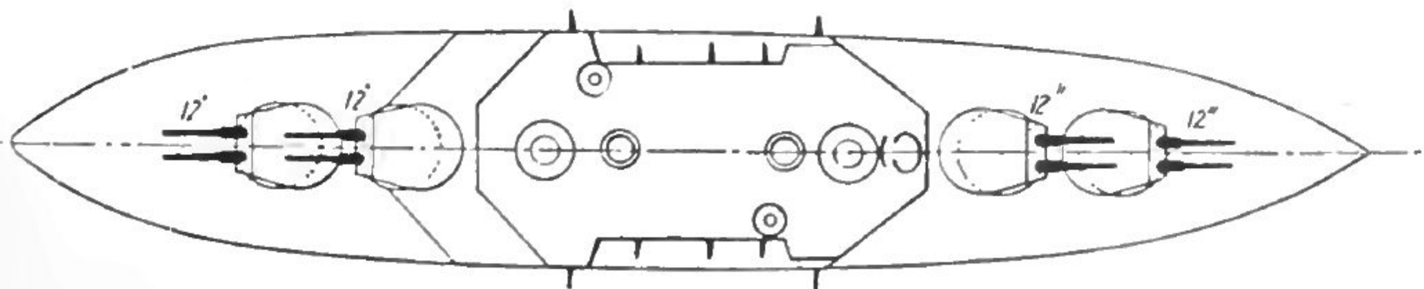
Length, 450 ft. ; 16,000 tons ; Speed, 18.5 knots ; Completed, 1909 ; Armament, 8—12 in., 22—3 in., 16 small.
