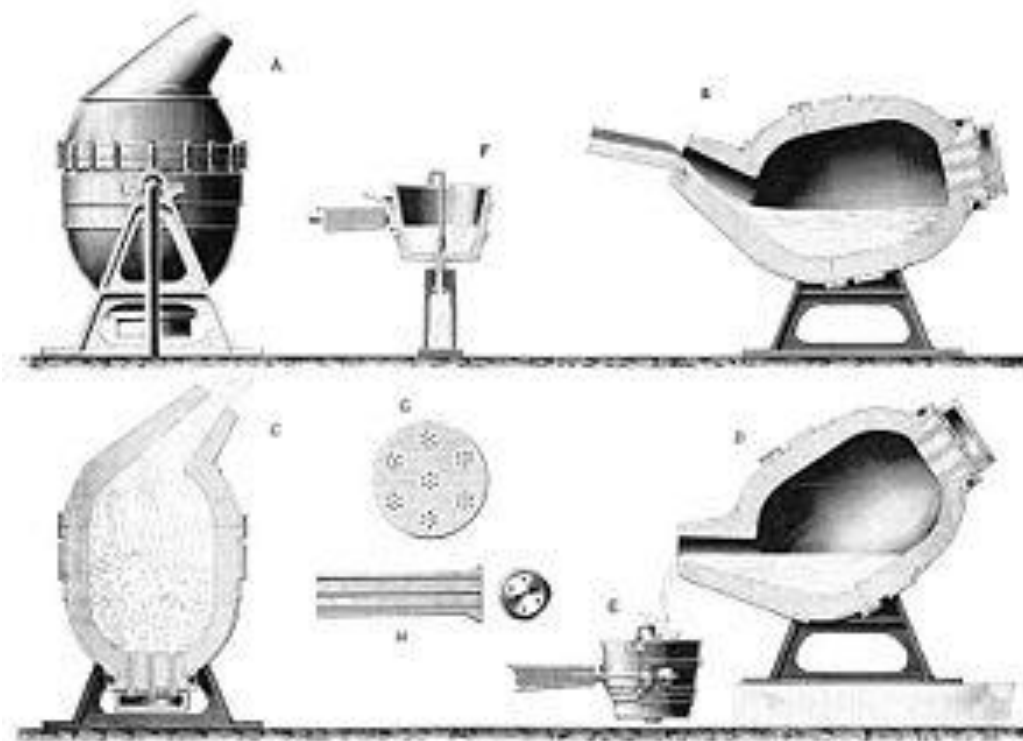
FIG. 65. THE PART-TAKE OF BESSEMER'S METHOD OF CONVERTING IRON INTO STEEL.
