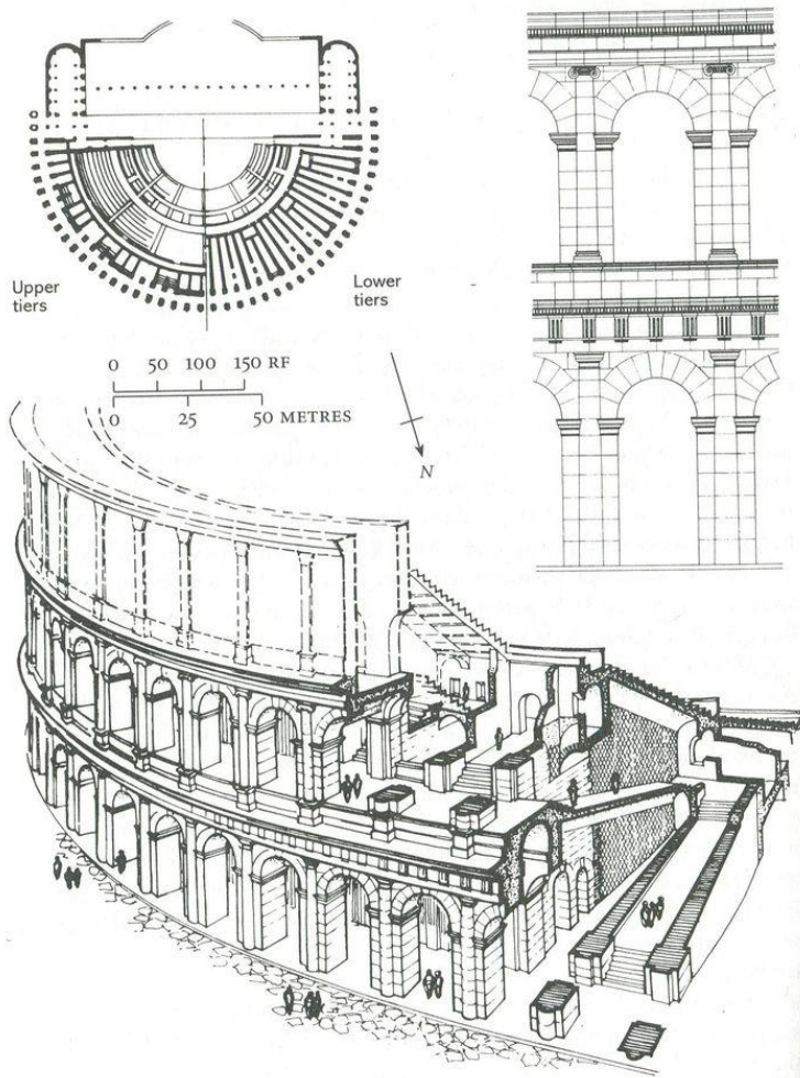
▲ Fig. 113. Theatre of Marcellus. Reconstructed plan, section of seating (cavea), and outer elevation
