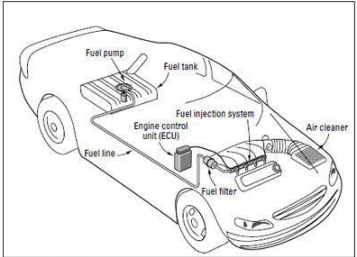
Figure 7-1: A fuel system.
