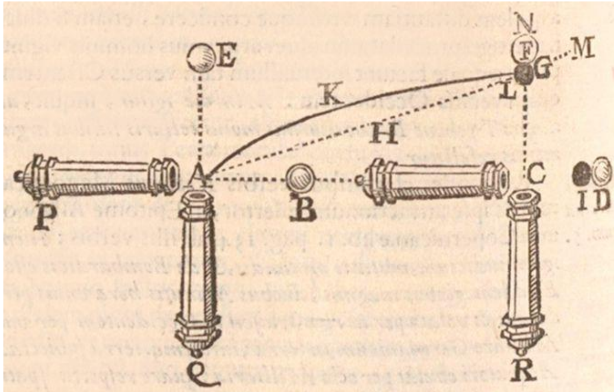
Illustration from Giovanni Battista Riccioli's 1651 Almagestum Novum . Because of Earth's rotation, a projectile fired north to hit a target at E/N follows curved path AKF, and strikes east of N at G. This effect is today referred to as the Coriolis effect, after the early 19th-century physicist.
