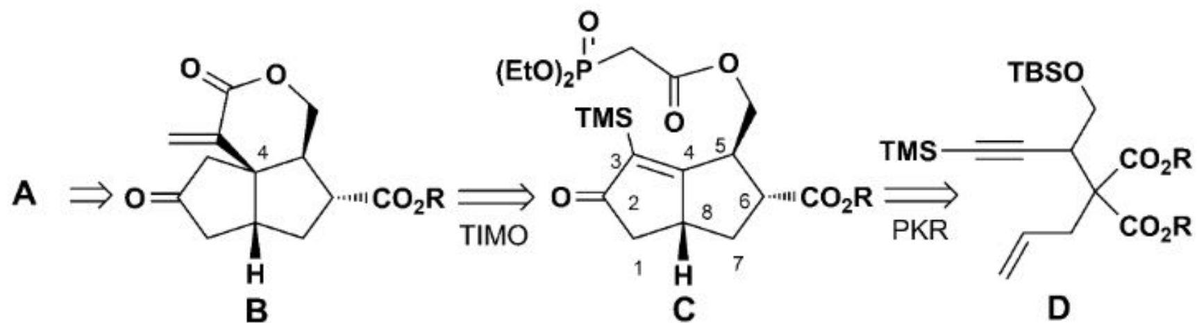
Scheme 2. Retrosynthetic analysis.
