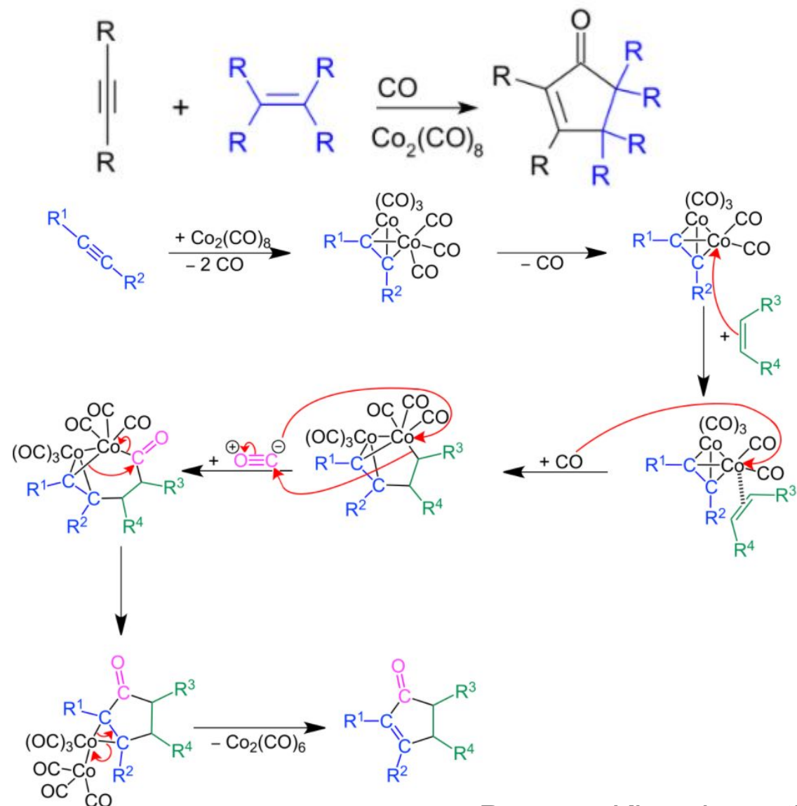
Pauson-Khand reaction
