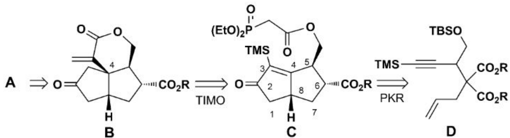
Scheme 2. Retrosynthetic analysis.
