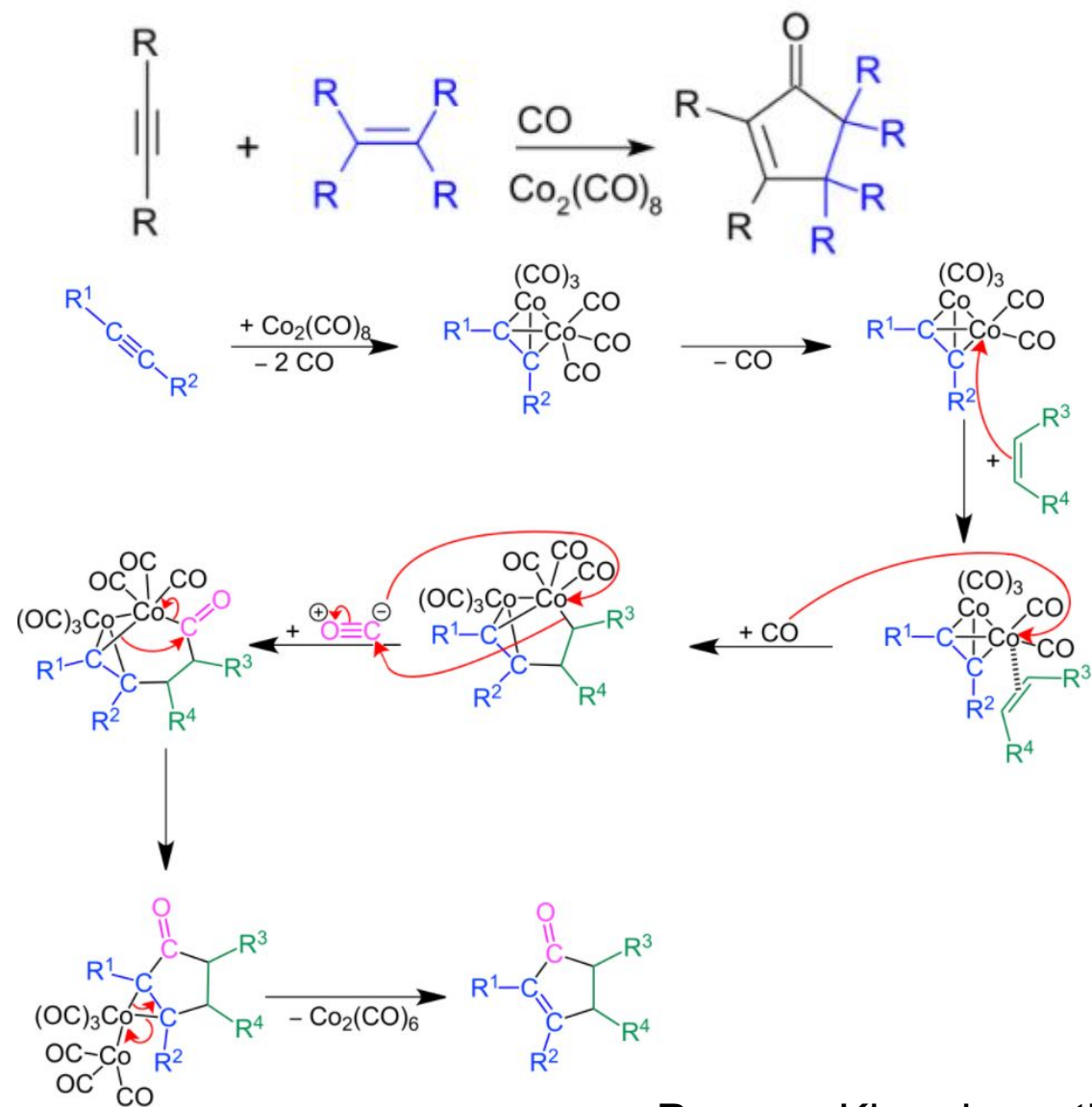
Pauson-Khand reaction
