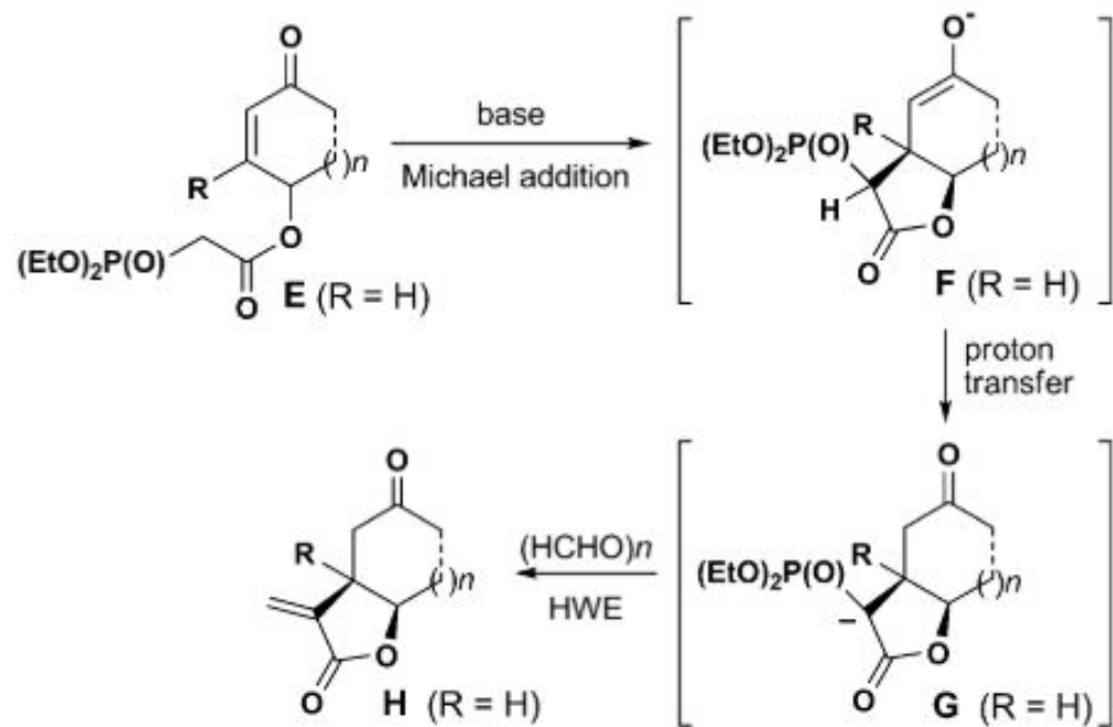
Scheme 4. Synthesis of \alpha -methylidene- \gamma -butyrolactones H . HWE = Horner–Wadsworth–Emmons reaction.
