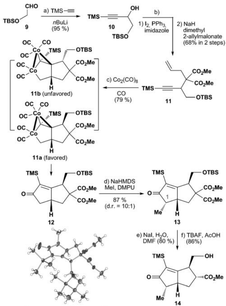
X-ray structure of compound 13
