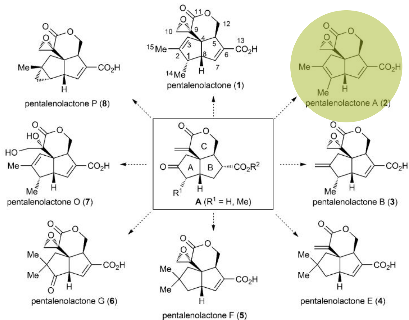
Scheme 1. Pentalenolactones and their synthetic relationship.
