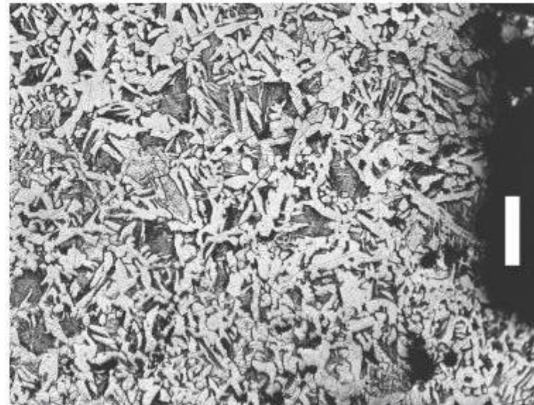
Fig. 2. The microstructure of helm DHM 1003; pearlite and ferrite (scale bar = 100 microns in each photomicrograph).
