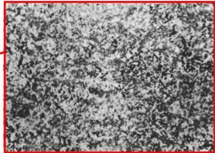
X 2000. Tempered martensite, showing a mass of tiny carbide particles
