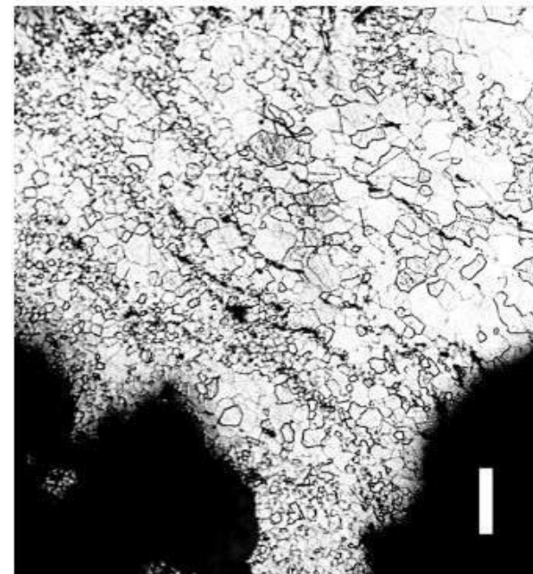
Fig. 4. The microstructure of helm Liestal 531.211; ferrite only.
