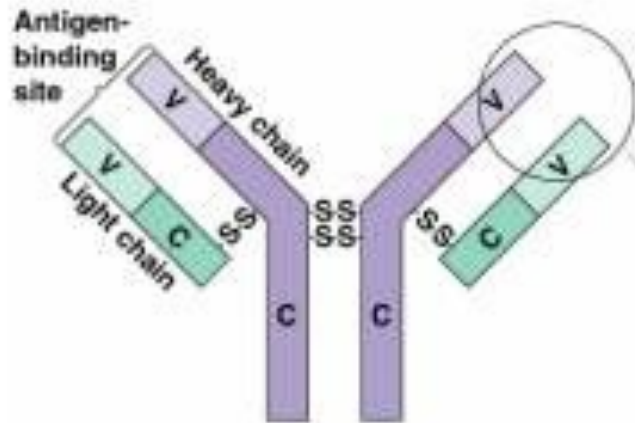
(a) Antibody molecule
