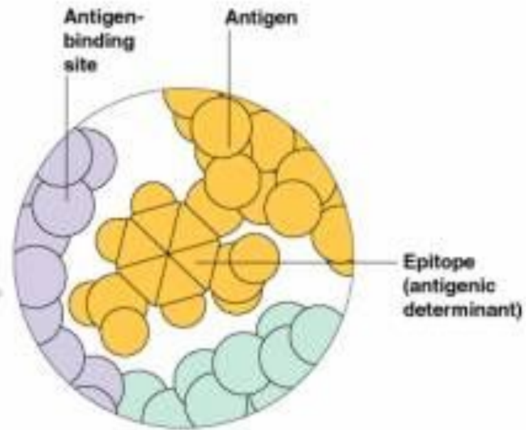
(b) Enlarged antigen-binding site
