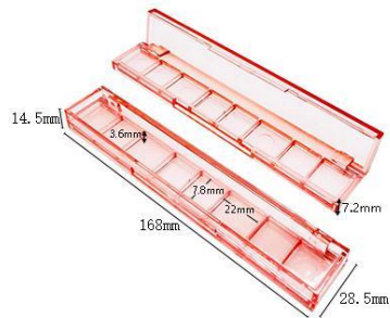
YSX-H4402 SIZE:W28.5*L168*H14.5MM
