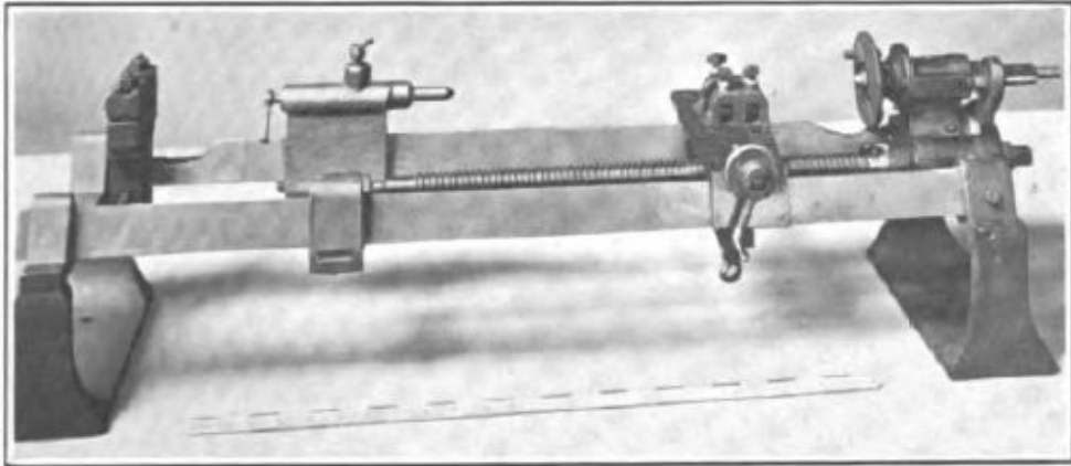
FIGURE 15. MAUDSLAY'S SCREW-CUTTING LATHE ABOUT 1797
