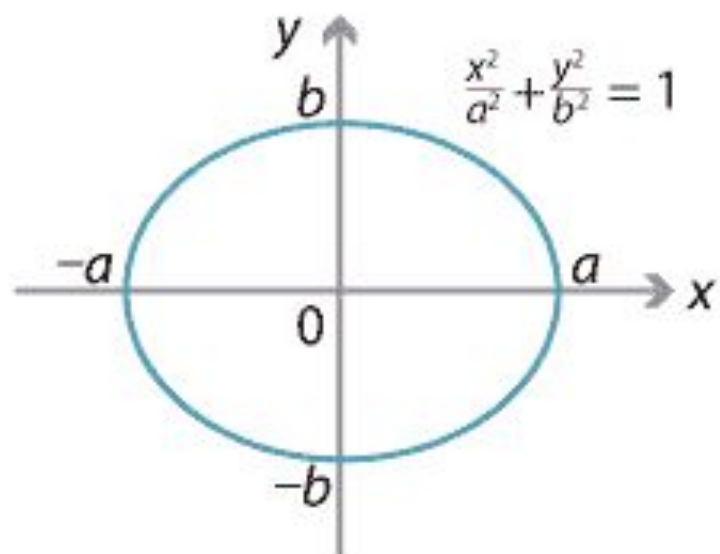
Ellipse
