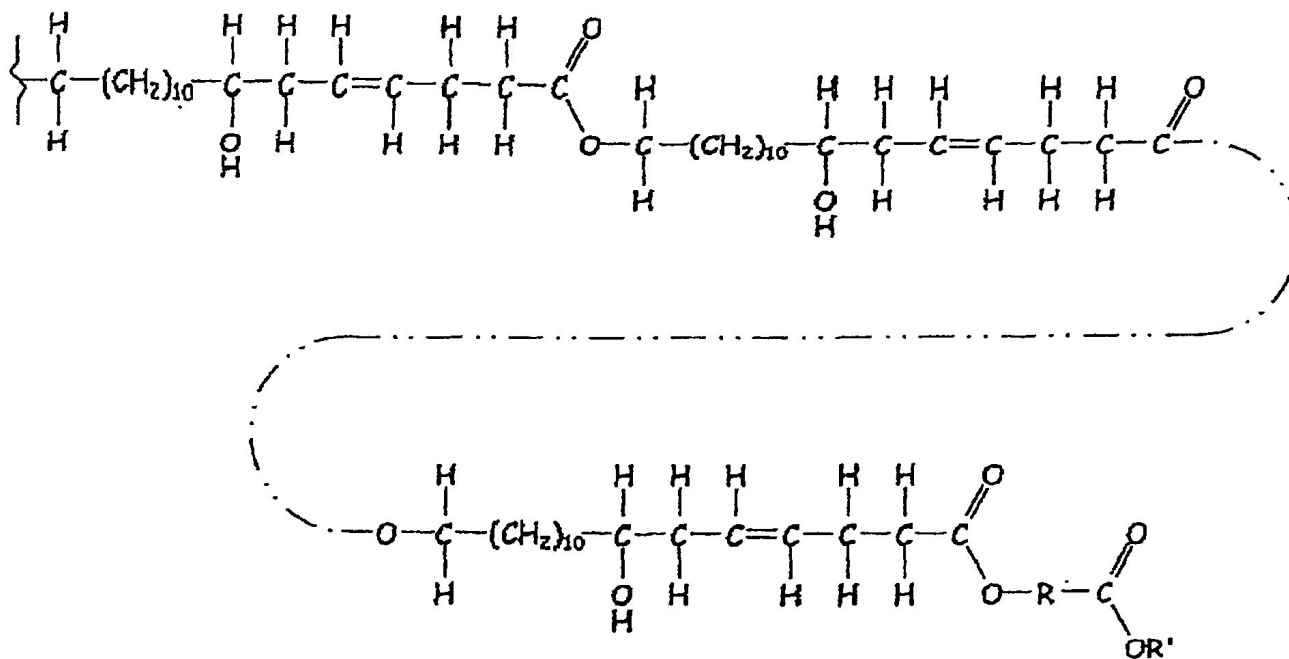
POLYMER ESTER OF RICINOLEIC ACID
