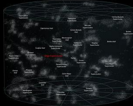
Local Superclusters
