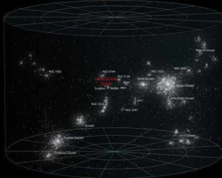
Virgo Supercluster
