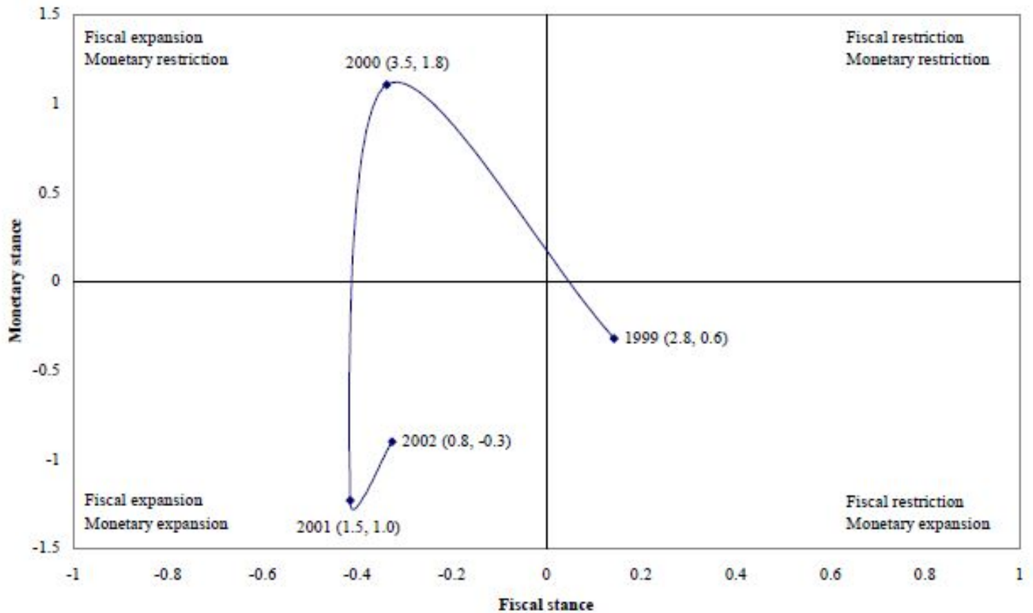
Figure 4.10 Euro area policy mix: 1999-2002
