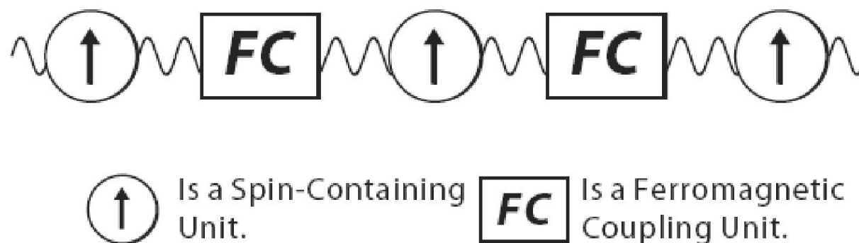
Figure 6.9: A schematic model for the design of high-spin organic molecules.
