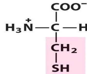
Цистеин (Cys)
