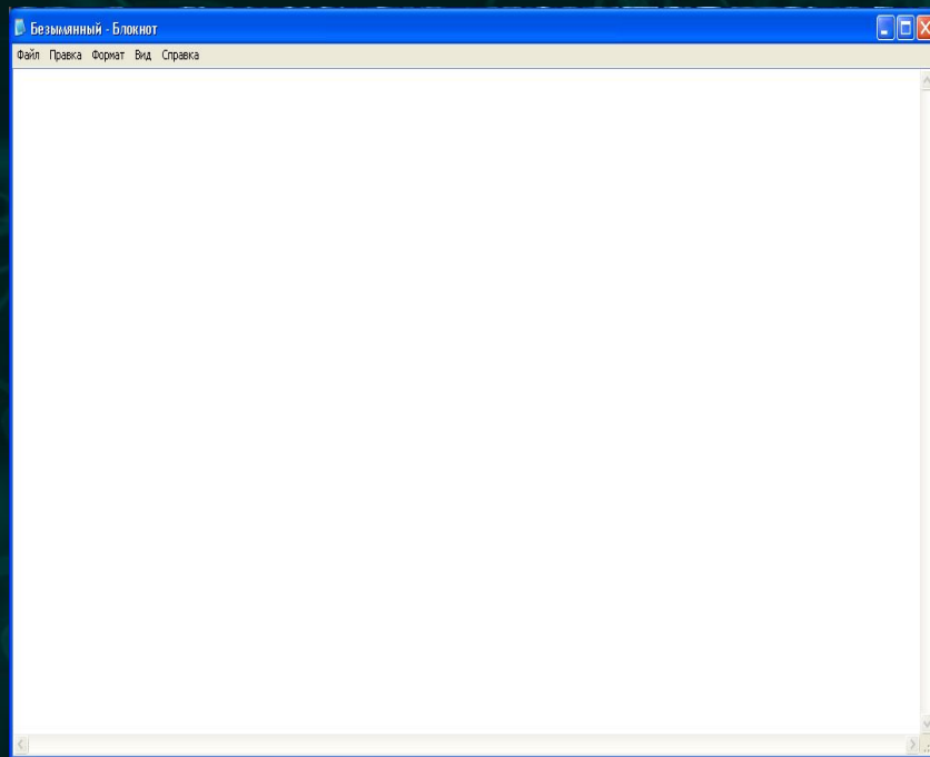
Windows Notepad
