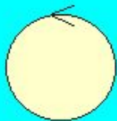
Control Class
