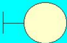
Boundary Class
