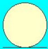
Entity Class
