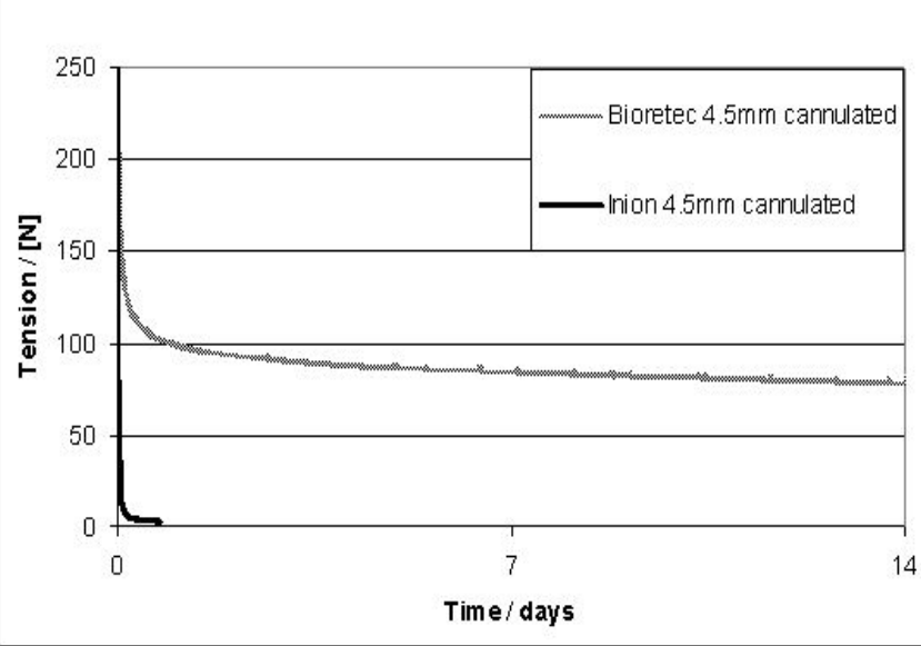
Stress Relaxation of Cannulated Screw
