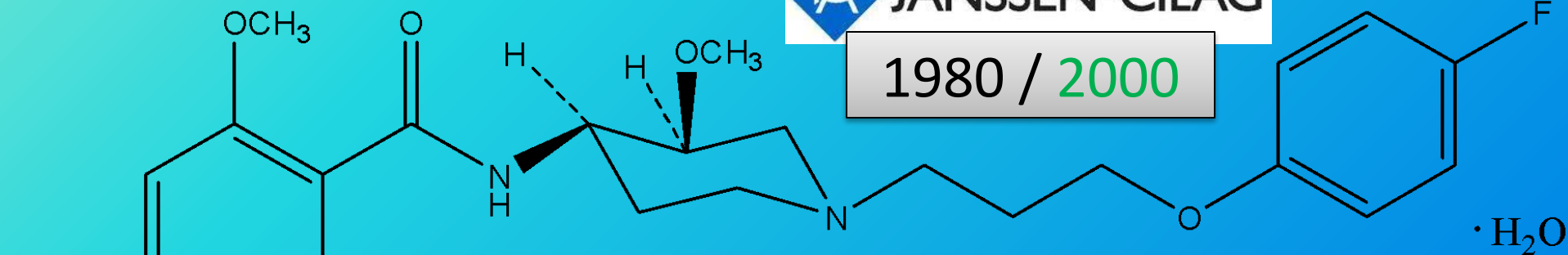
Cisapride Monohydrate
