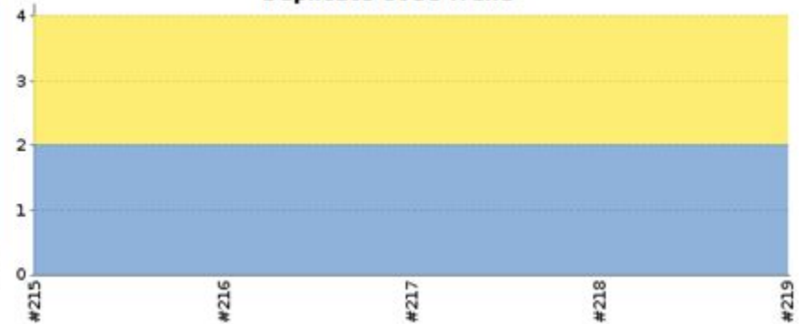
Checkstyle Trend
