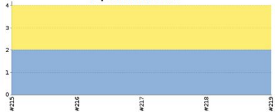
Checkstyle Trend
