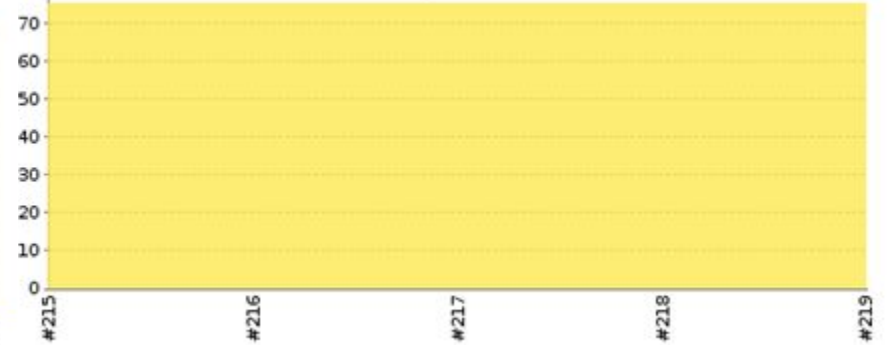
Checkstyle Trend
