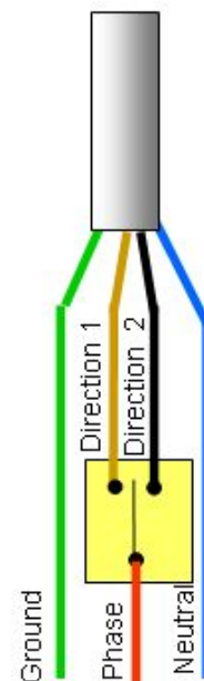
AC switching
