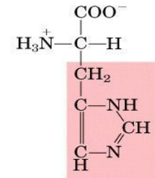
Histidine
