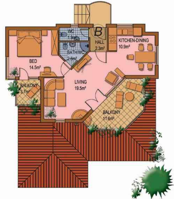
SECOND FLOOR M 1:100
