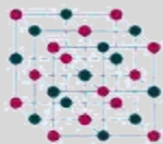
Sodium Chloride
