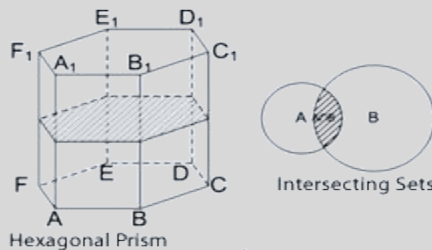
Hexagonal Prism
