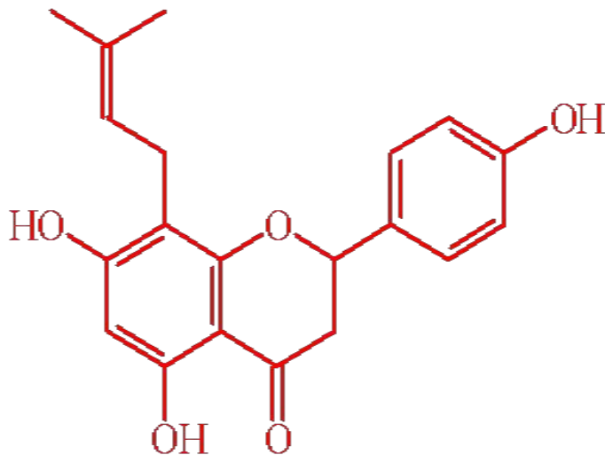
8-Prenylnaringenin
