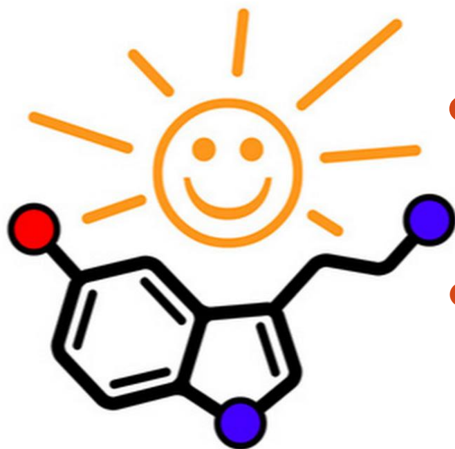
serotonin
