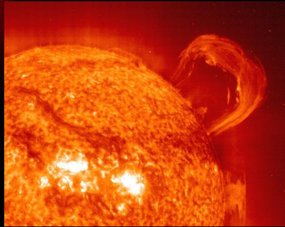
Solar prominences
