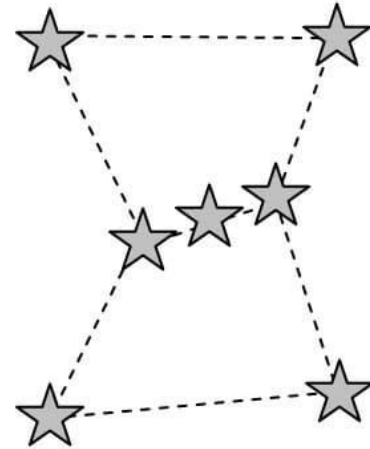
Orion constellation
