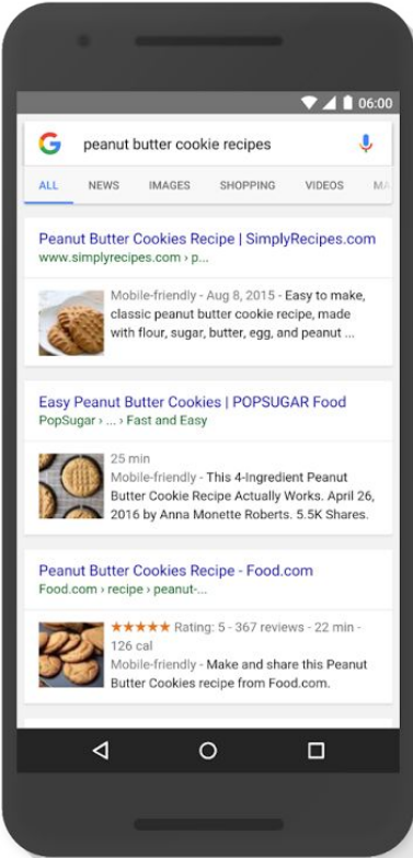
Rich Snippets
