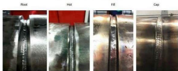
GTAW+FCAW example
