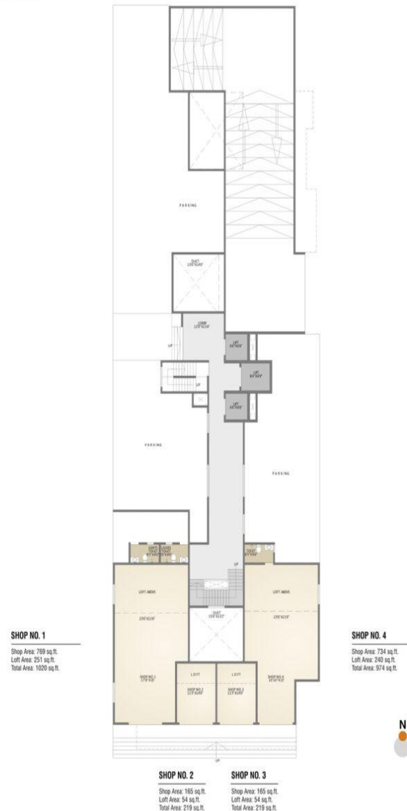
GROUND FLOOR PLAN BUILDING A
