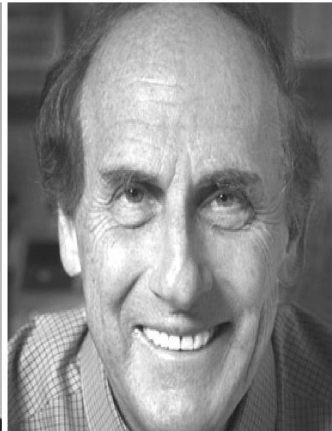
RALPH STEINMAN
