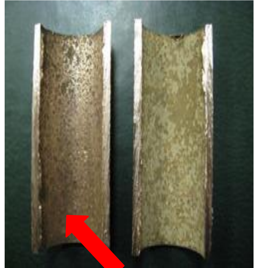
Corrosion appeared after scale deposit
