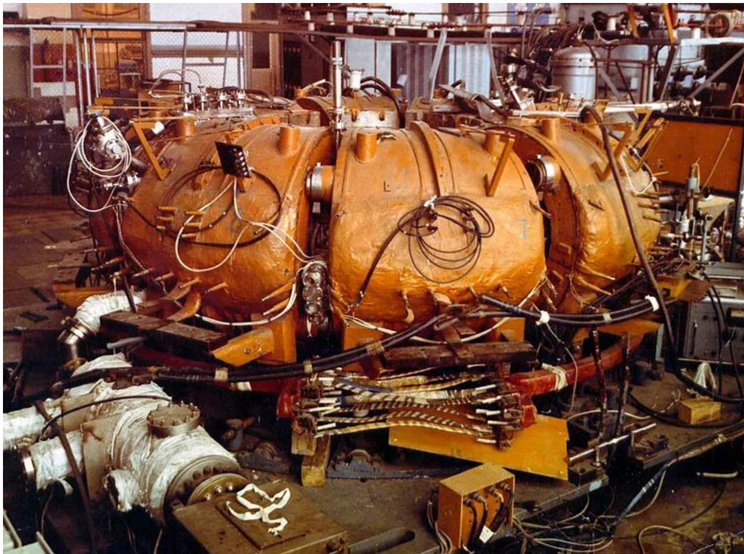
TOKAMAK "TM-3"
