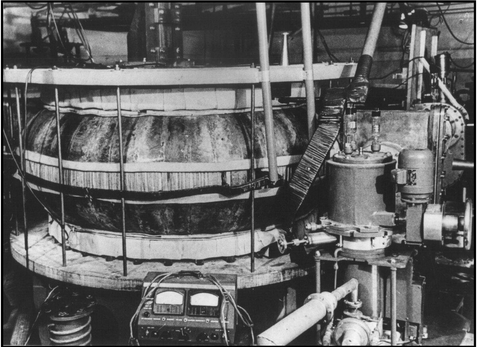
TOKAMAK T-1
