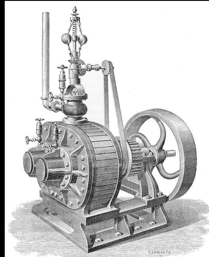
Fig. 323.—Behren's Rotatory Engine.
