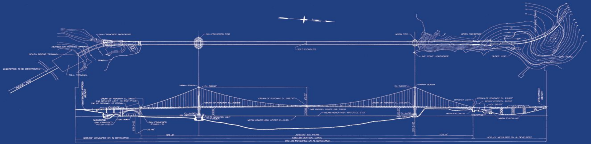
THE GOLDEN GATE BRIDGE SAN FRANCISCO, CAL. MAIN BRIDGE PLAN AND ELEVATION SCALE IN FEET
