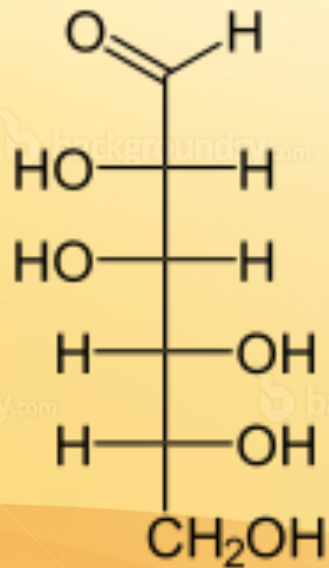
D-Mannose
