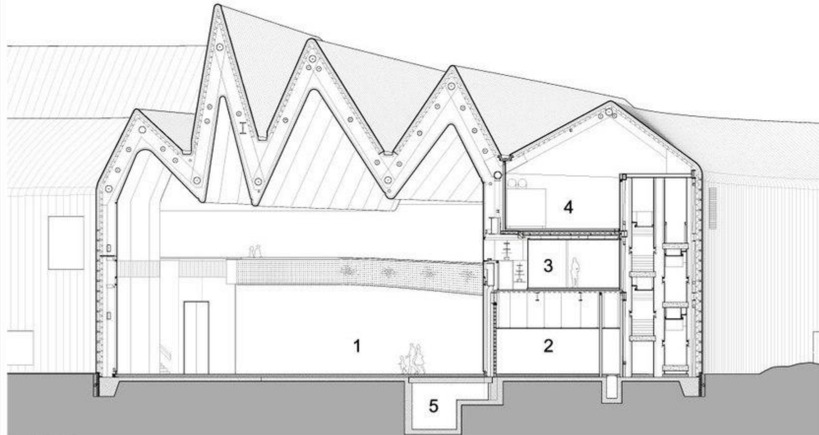
2 SECTION H - H
