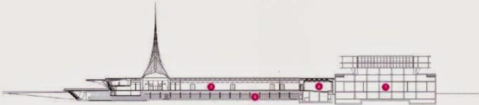
North-South Section
