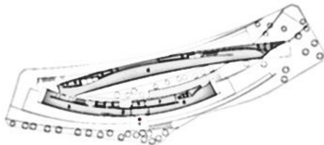
● 1 st FLOOR Scale 1/ 1000 1 : Entrance 2 : Museum shop 3 : Entrance hall 4 : Gallery (1) 5 : Machine room 6 : Restaurant 7 : Kitchen
