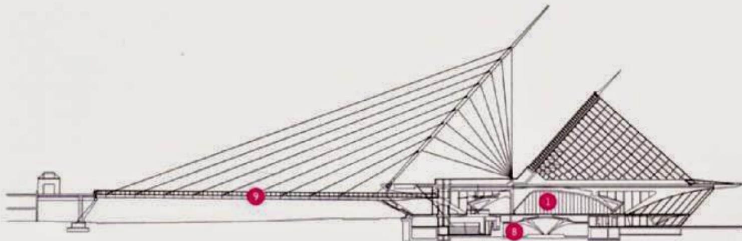
North-South Section
