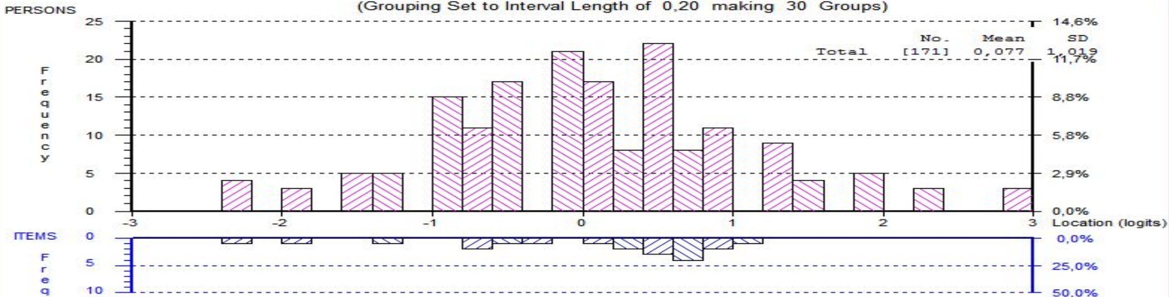
Person-Item Location Distribution (Grouping Set to Interval Length of 0,20 making 30 Groups)
